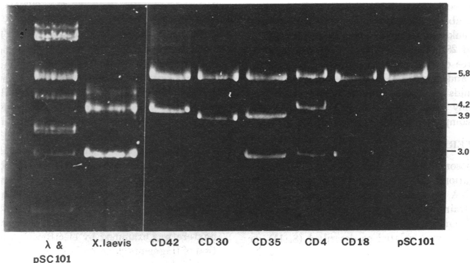
FIG. 2. Agarose gel electrophoresis of fragments generated by EcoRI endonuclease. DNA was isolated and digested to completion with excess EcoRI endonuclease. Electrophoresis was in a 0.7% agarose slab gel (17 cm \times 13 cm \times 3 mm) at 3 V/cm in 0.09 M Tris base–2.8 mM EDTA–0.09 M boric acid (pH 8.3) buffer at 25° for 15 hr. After completion of electrophoresis, the DNA was stained with 4 \mu\text{g/ml} of ethidium bromide and photographed under a long-wave UV lamp (refs. 1, 6, and 18; Helling, Goodman and Boyer, in preparation). Electrophoresis was from top to bottom in the figure (i.e., the anode is at the bottom) and the source of DNA is indicated. The figure shown is a composite of two separate gels. An EcoRI endonuclease digest of a mixture of bacteriophage \lambda DNA and pSC101 DNA was used for molecular weight standardization, and is shown in the left-hand column. The bands seen in this column had estimated molecular weights (counting from the bottom): 2.09, 3.03, 3.56, 3.7, 4.7, 5.8 (pSC101), 13.7, and 15.7, all \times 10^6 (Helling, Goodman and Boyer, in preparation). The 15.7 \times 10^6 fragment results from joining of the terminal cohesive ends of \lambda DNA, which are located on the 2.09 and 13.7 \times 10^6 fragments. The calculated molecular weights of the major fragments present in X. laevis rDNA treated with EcoRI endonuclease and in the plasmids shown are indicated in the figure. All values have been multiplied by 10^6 .
